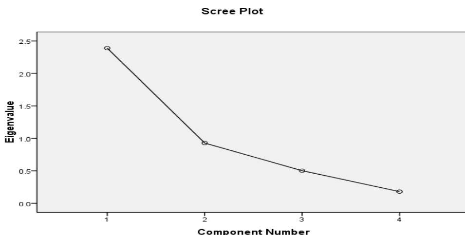
Figure 5: Showing the Scree Plot graph.
