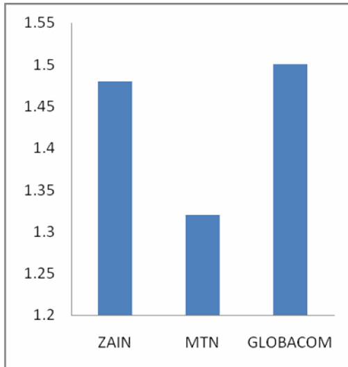
Figure 3(a): Average power density at 100cm
