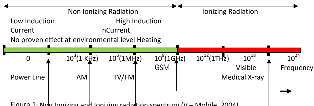
Figure 1: Non Ionizing and Ionizing radiation spectrum (V – Mobile, 2004)
